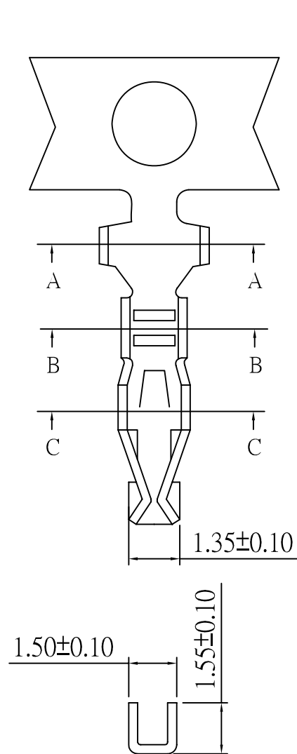
C-C SECTION
