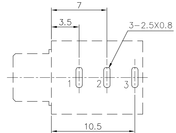
T:1.6 Dimensions of PC board holes
