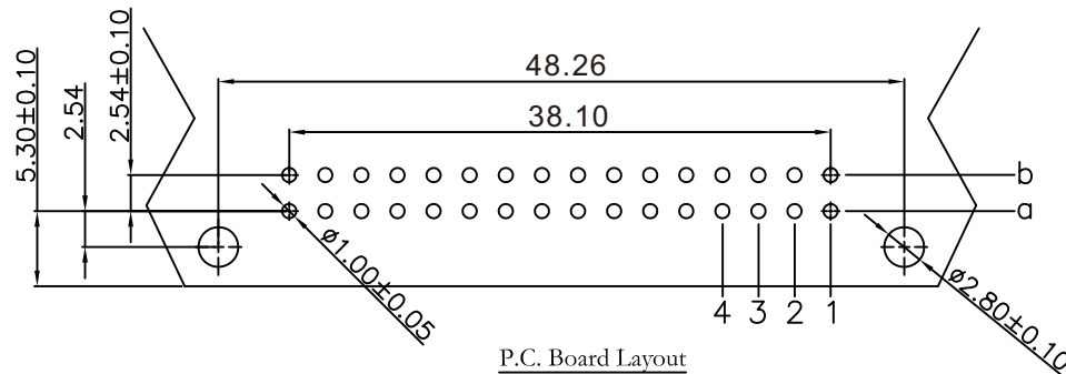
P.C. Board Layout
