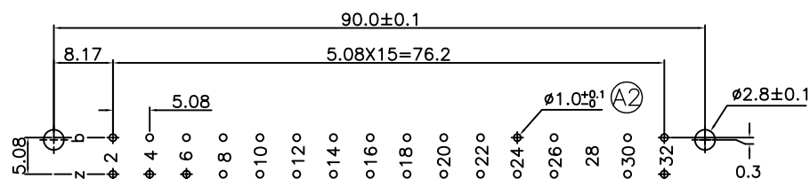
P.C. Board Layout
