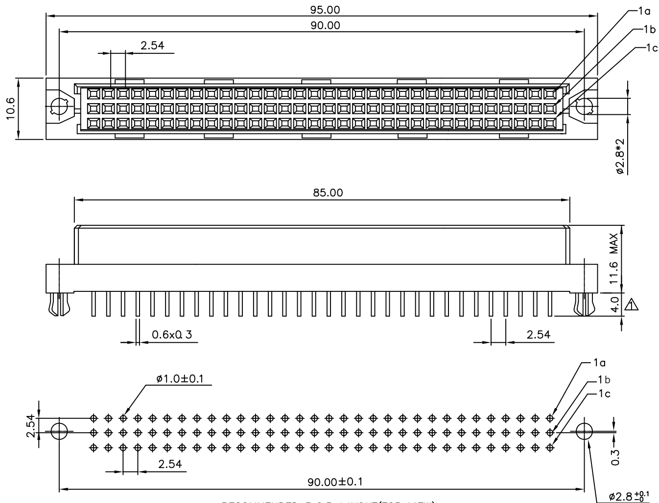
RECOMMENDED P.C.B LAYOUT(TOP VIEW) TOLERANCES: \pm 0.10\text{mm}
