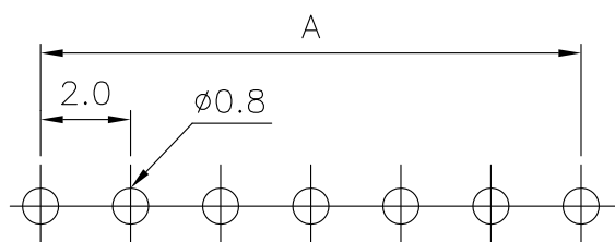
PCB HOLE LAYOUT
