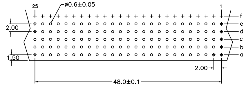
P.C. Board Layout (Top View)
