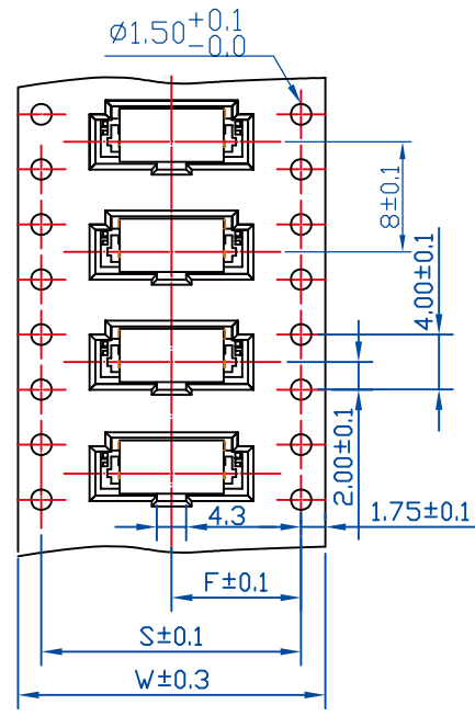
14~16P&20P Contacts
