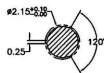
DETAIL J
