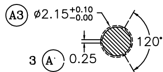
Detail J (Scale 5 : 1)
