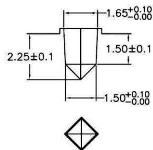
DETAIL K
