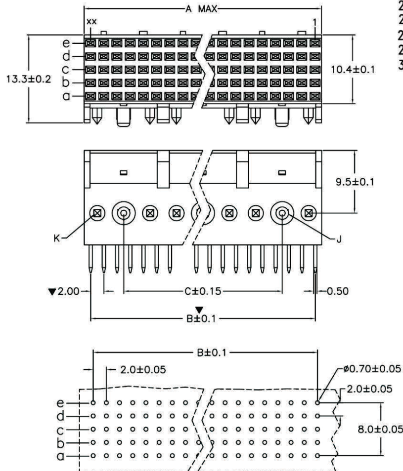
P.C. Board Layout
