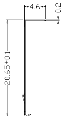
Bottom Shielded
