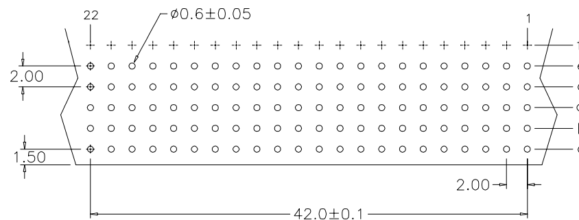
P.C. Board Layout (Top View)
