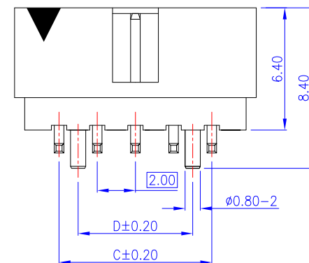
10 Pin
