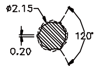
Detail J (Scale 5 : 1)
