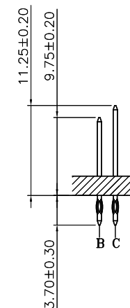
CONTACT LAYOUT
