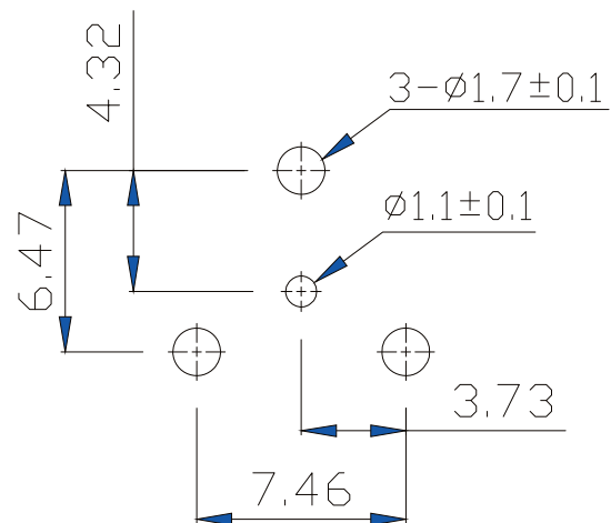
PCB HOLE CONFIGURATION RECOMMENDED PANEL CUTOUTS
