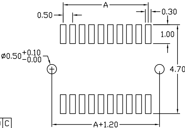
Recommended PCB Layout (PCB TOLERANCE ±0.08)
