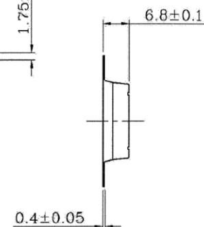
DETAIL "Y"
