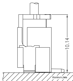
Assembly Layout
