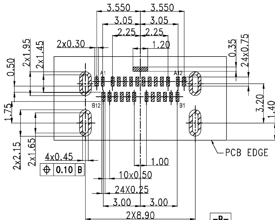
RECOMMENDED PCB LAYOUT (Tolerance=±0.05)
