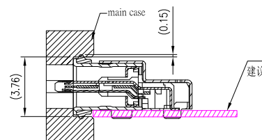
SECTION A-A PANEL CUT-OUT REFERENCE
