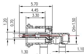
SECTION C-C(SC 1:1)
