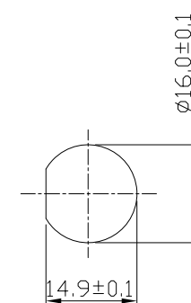
Recommend Panel Cut-Out
