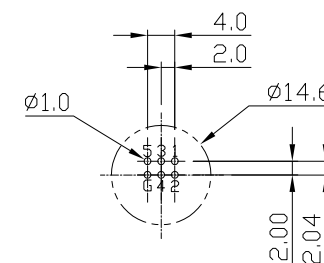
Recommend PCB Layout
