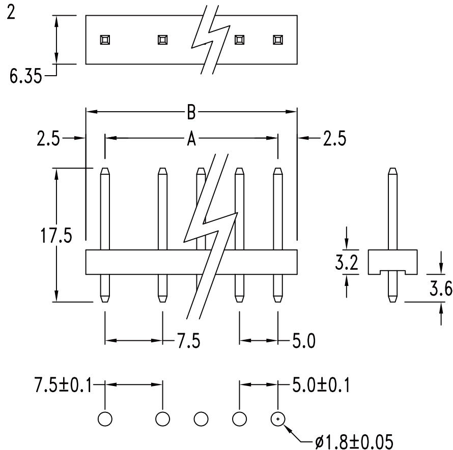
P. C. Board Hole Dimensions
