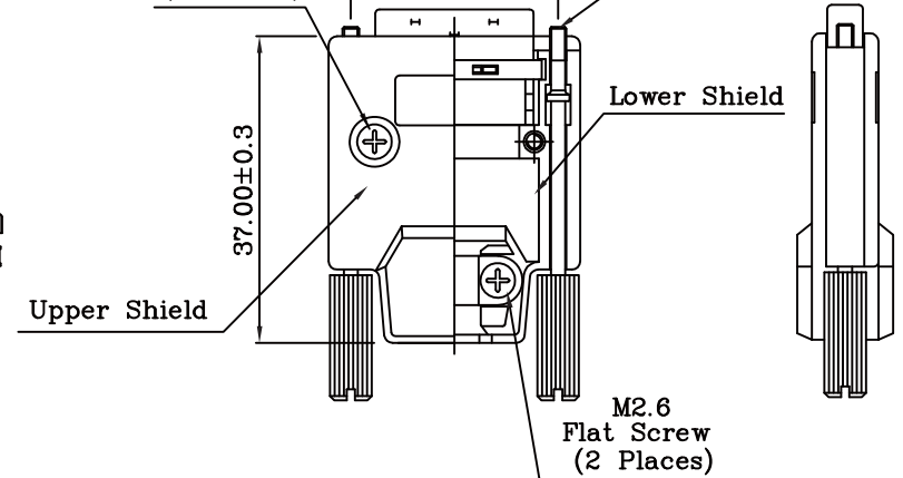
M2.6 Flat Screw (2 Places) M2.0 Jack Screw (2 Places)
