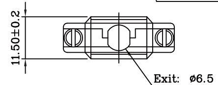
Cable Clipper
