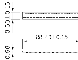
Wire Holder (2 Places)
