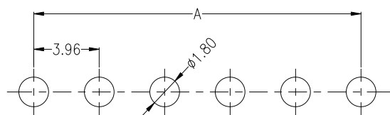
RECOMMENDED PCB LAYOUT(TOP VIEW) TOLERANCE: \pm 0.05\text{mm}
