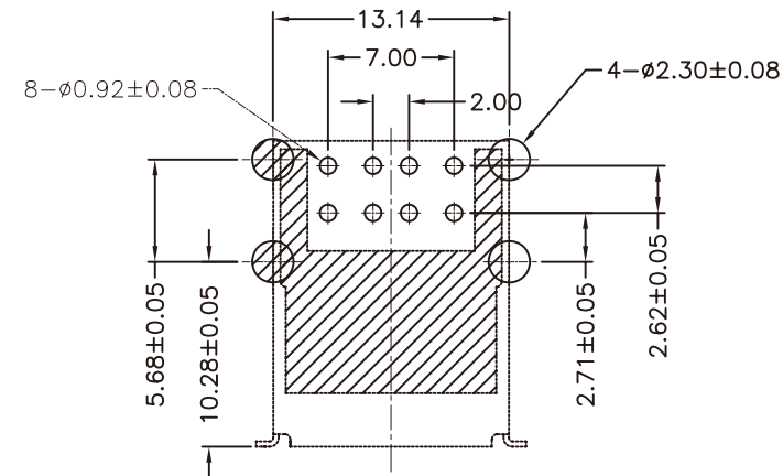
RECOMMEND P.C.Board HOLE LAYOUT
