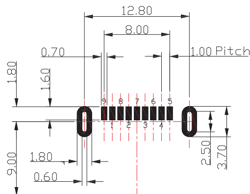
PCB EDGE RECOMMENDED PCBA LAYOUT
