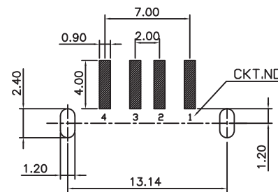
P.C.B LAYOUT TOLERANCE:±0.10
