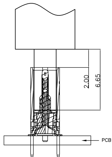
AFTER MATING
