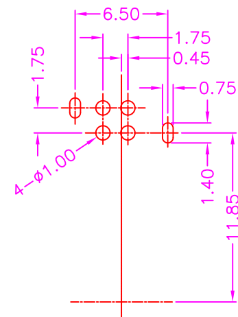
P.C.B. LAYOUT TOP VIEW \pm 0.05
