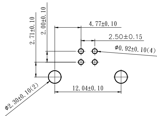
RECOMMENDED P. C. B. PATTERN LAYOUT
