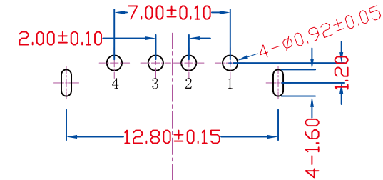
FRONT EDGE OF CONNECTOR PCB LAYOUT (T=1.60mm)
