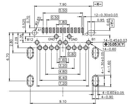
RECOMMENDED PCB LAYOUT(TOP VIEW) (TOLERANCE=±0.05mm)
