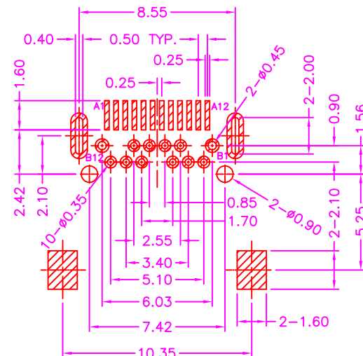
P.C.B. LAYOUT TOP VIEW±0.05
