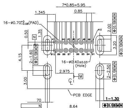
ECOMENDED P.C.B LAYOUT
