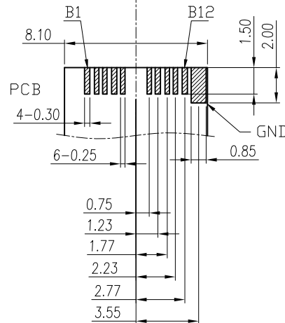
RECOMMEND PCB LAYOUT BOTTOM VIEW
