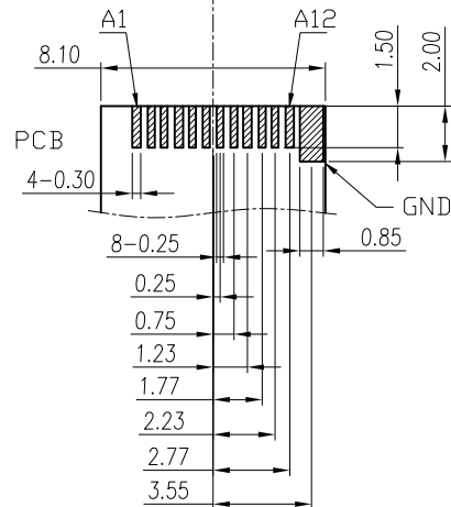
RECOMMEND PCB LAYOUT TOP VIEW
