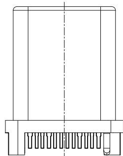
Connector TOP VIEW
