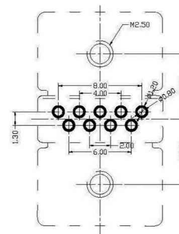
PCB LAYOUT
