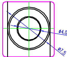
CABLE EXIT: TYPE I (RECOMMENDED CABLE OD= \phi 3.4~ \phi 3.8)
