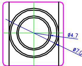
CABLE EXIT: TYPE II (RECOMMENDED CABLE OD= \phi 3.9~ \phi 4.6)
