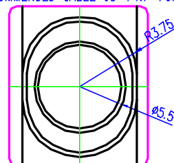
CABLE EXIT: TYPE III (RECOMMENDED CABLE OD= \phi 4.7~ \phi 5.3)
