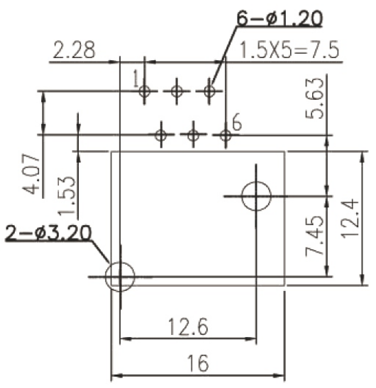
PCB LAYOUT
