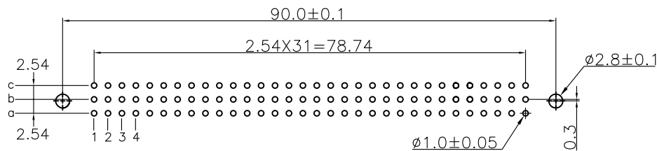
P.C. Board Layout
