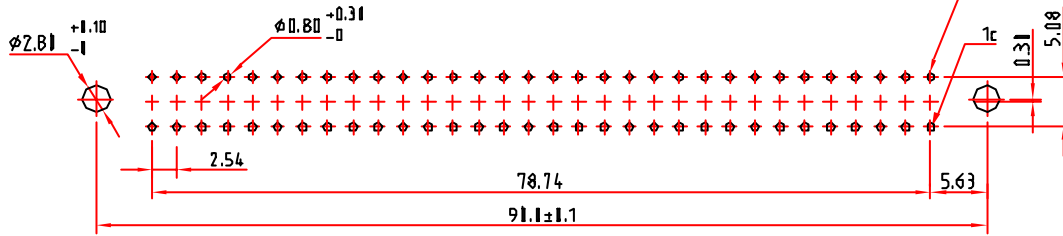
RECOMMENDED P.C. BOARD LAYOUT
