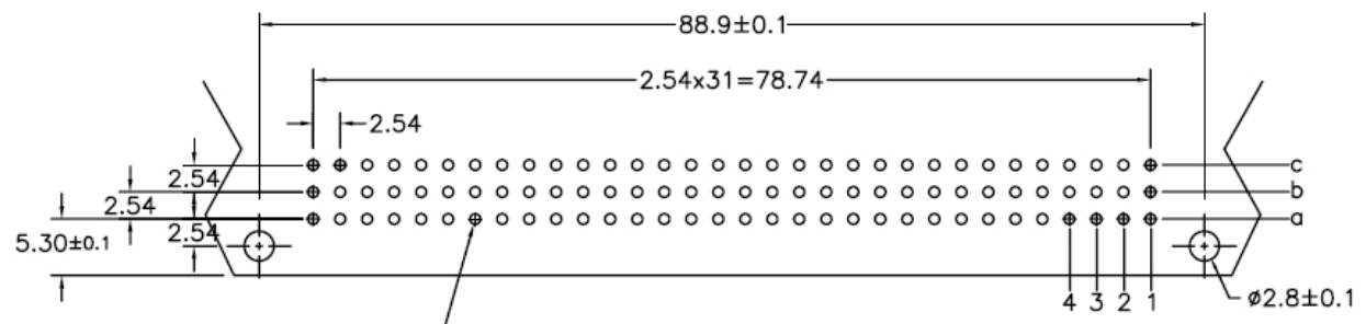
P.C. Board Layout (Tolerance:±0.05)
