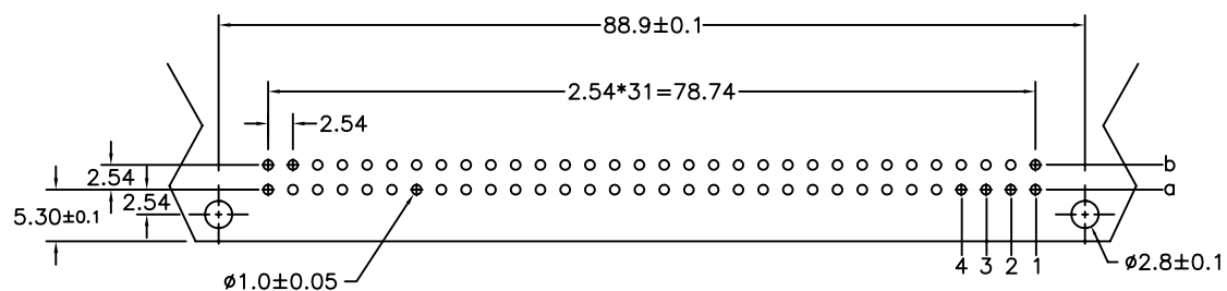
P.C. Board Layout (Tolerance: \pm 0.05 )
