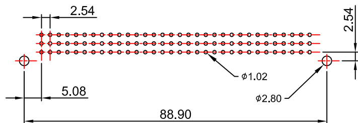
PCB LAYOUT
