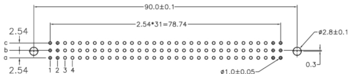
P.C. Board Layout
