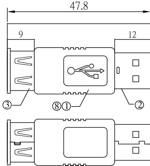
P1 USB A TYPE FEMALE
