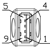
CONN.#1
