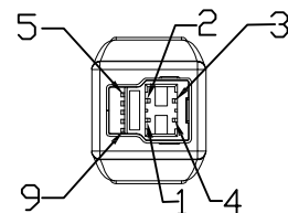
CONN.#2
