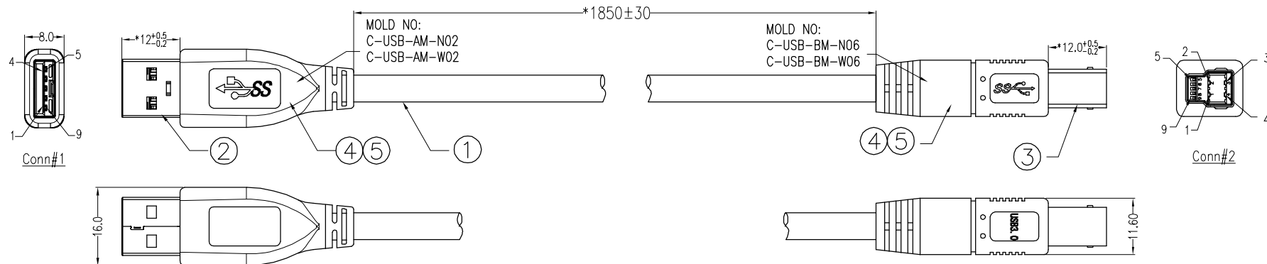
Pin Assignment
