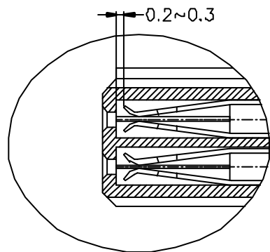
B-B' VIEW
