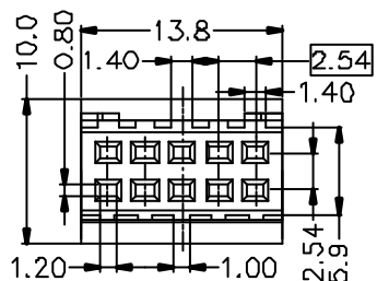
B-B' VIEW
